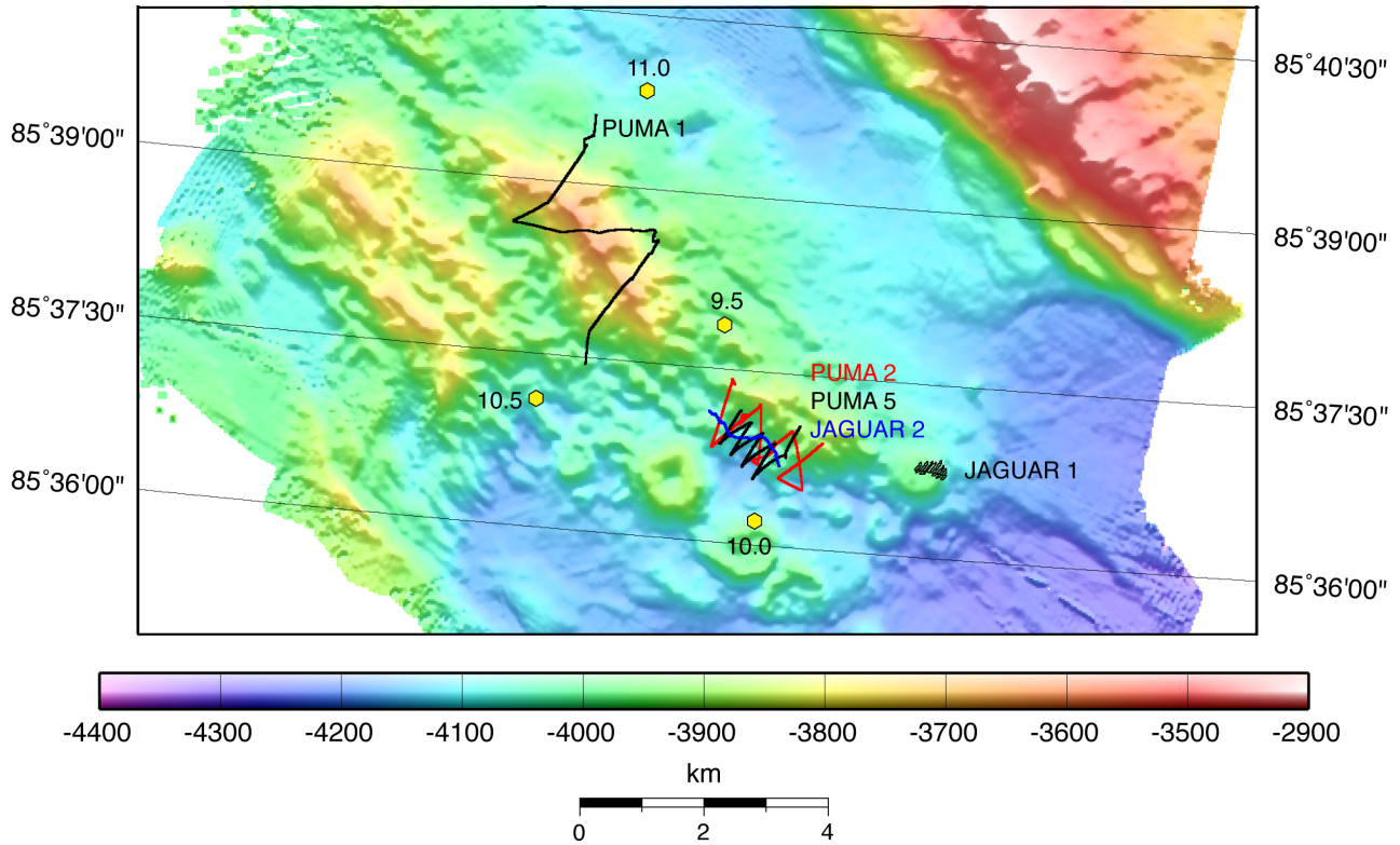
Fig. 4. Actual tracklines flown during AUV missions superimposed on local bathymetry. This figure does not include the single Puma dive performed at a separate divesite at 85°N, 7°E.
